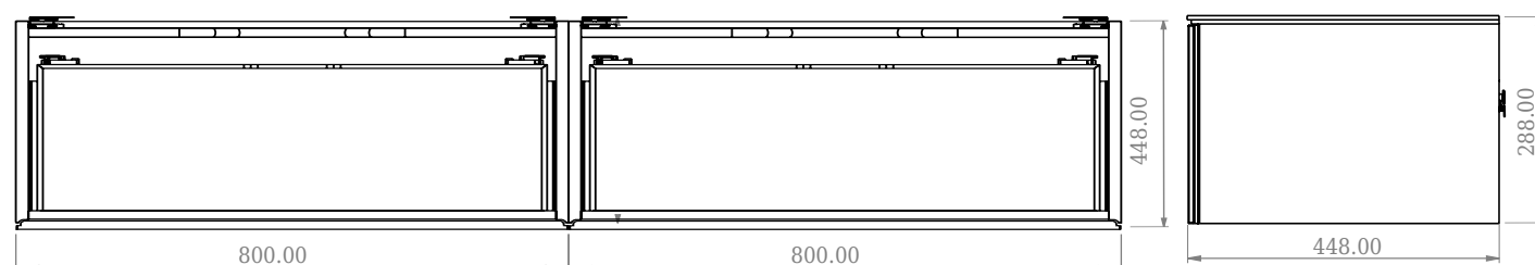
Side View
